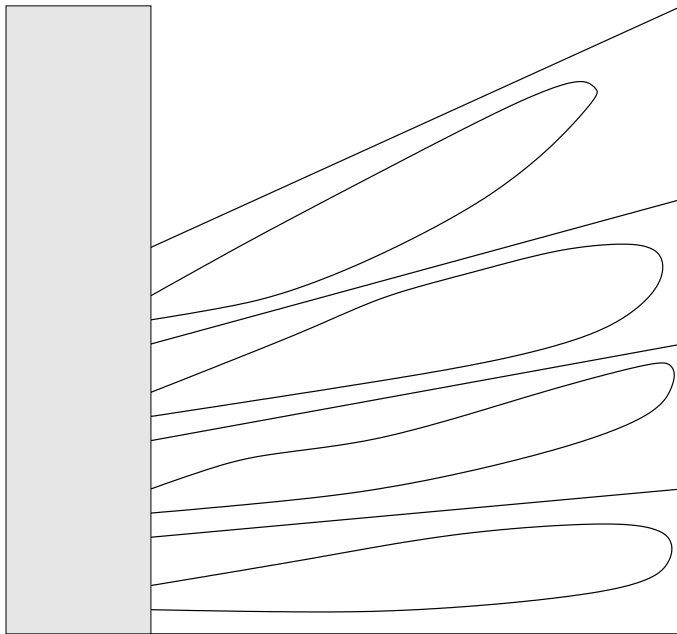
Figure 2: A set of disjoint wedges.
