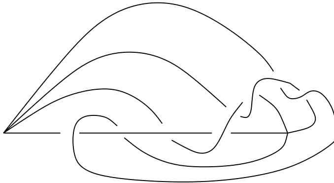
Figure 1: An almost unknotted \Theta_4 graph.
